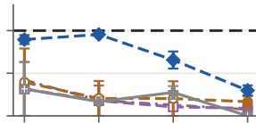
Max. degree 3 graphs
