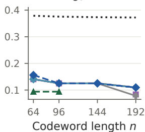
\log_3 M/n
