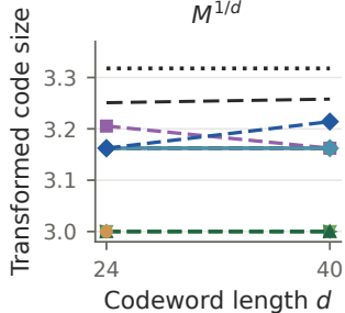
M^{1/d}
