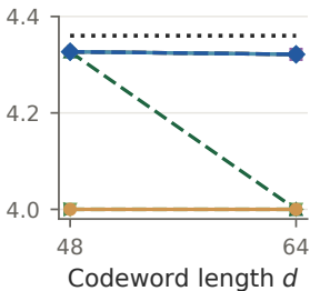
M^{1/d}
