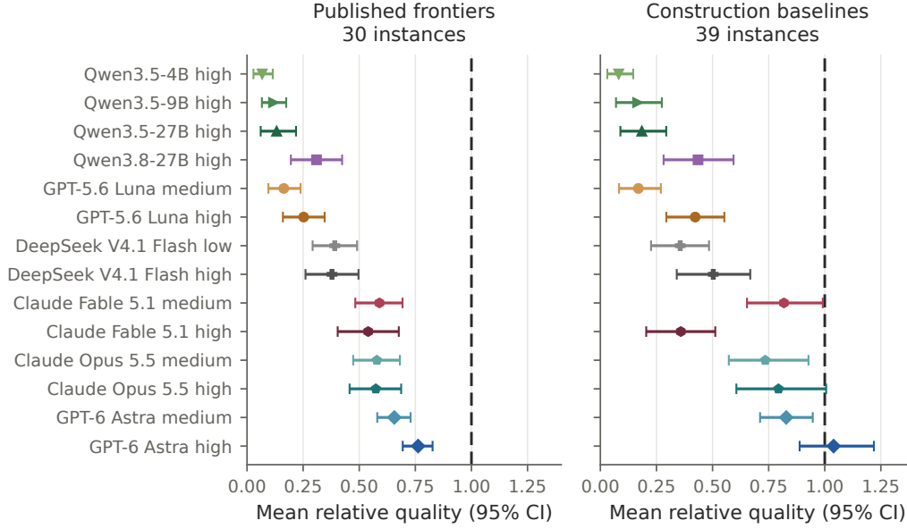
Figure 6: Fourteen-family construction quality for all fourteen tool-free configurations. Whiskers show 95% confidence intervals obtained by resampling instances within each reference group: 30 with published frontiers and 39 with construction baselines.
