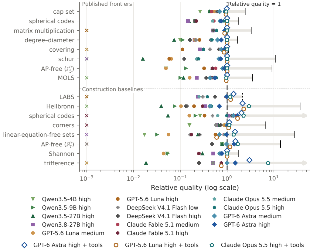
Figure 2: Mean relative quality across fourteen families. Model points and bar endpoints are normalised to the reference and averaged over the same instances in each row; model means include zero scores. Upper rows use published frontiers; lower rows use construction baselines. A ratio of 1 matches the reference. Grey bars extend from the reference level of 1 to mathematical bounds or conjectured targets. A solid mark at the right end indicates a proven bound; a dashed mark indicates a conjectured target. An arrow means the endpoint lies beyond the plotted range. Filled markers indicate tool-free evaluations and hollow markers tool-assisted evaluations. Crosses mark means below 0.001. AP-free: arithmetic-progression-free; LABS: low-autocorrelation binary sequences; MOLS: mutually orthogonal Latin squares.
