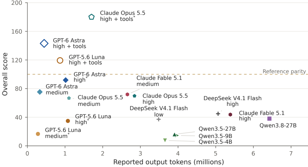
Figure 3: Overall score and output tokens for 69 instances, including reasoning and all model turns. For models marked with an asterisk, some output-token counts are unavailable, so the plotted totals are lower bounds. All Qwen models use high effort; tokenisation varies by model.
