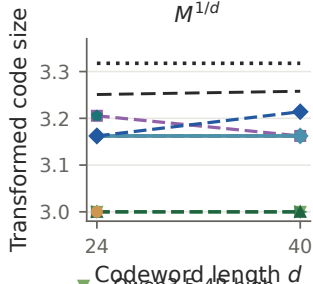
M^{1/d}
