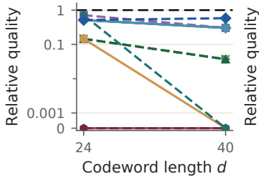
Shannon C_7 2 sizes
