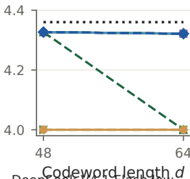
M^{1/d}
