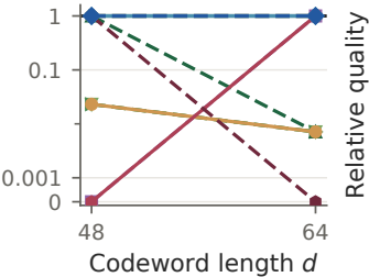
Shannon C_9 2 sizes
