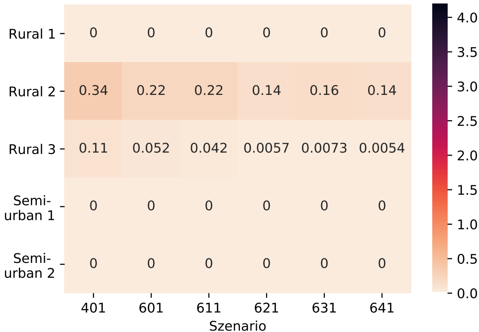
Curtailed load energy in MWh
