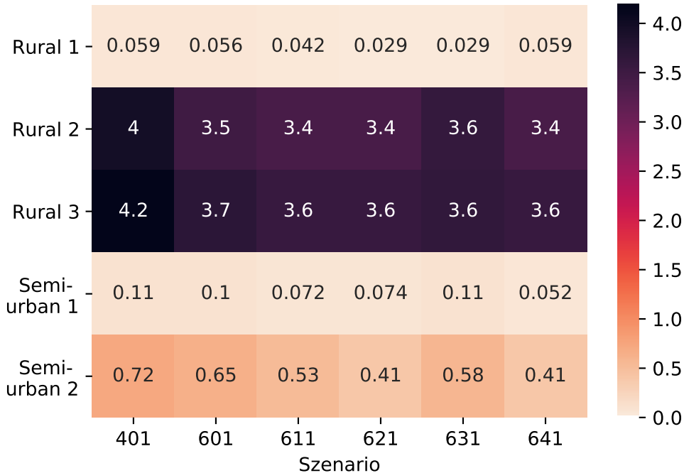
Curtailed pv energy in MWh
