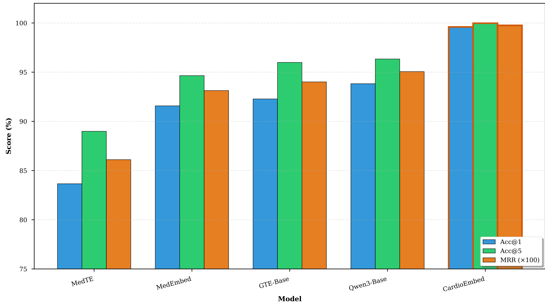
Performance Comparison Across All Metrics
