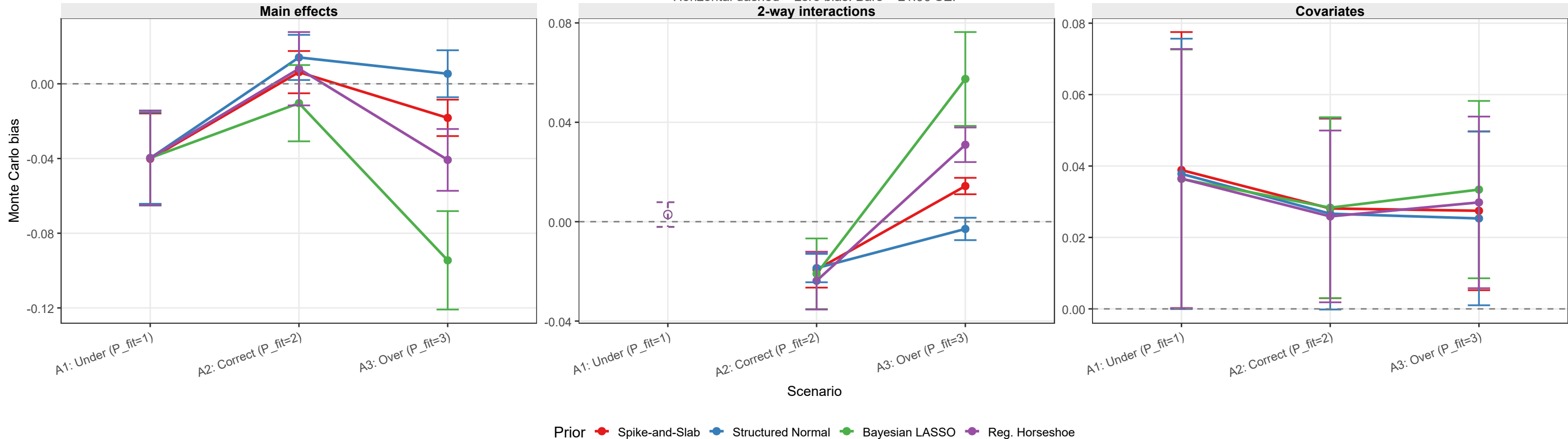
Figure b — Bias by parameter type, scenario, and prior
