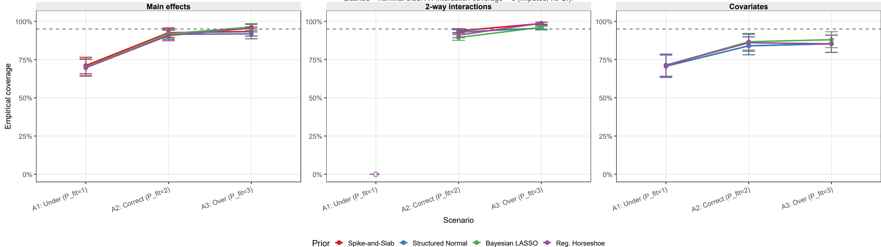
Figure c — 95% CI coverage by parameter type and scenario
