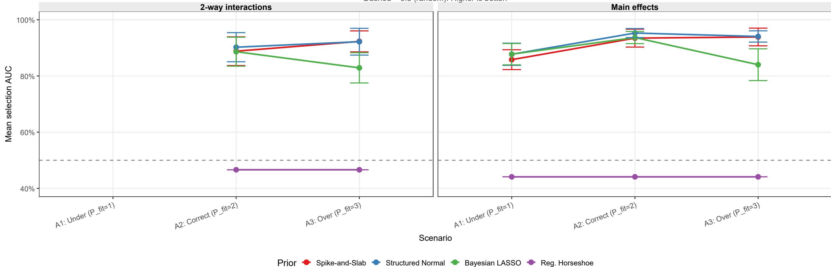
Figure c — Selection AUC (PIP score vs true non-zero)
