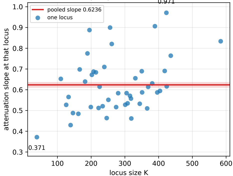
Per-locus slope spans 0.371-0.971 (2.6-fold)
