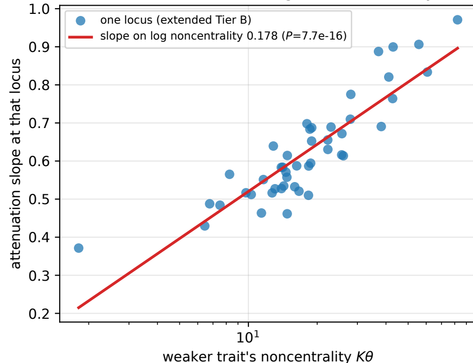
Channel 2 selects on power: survivors skew toward less-attenuated, higher-noncentrality loci
