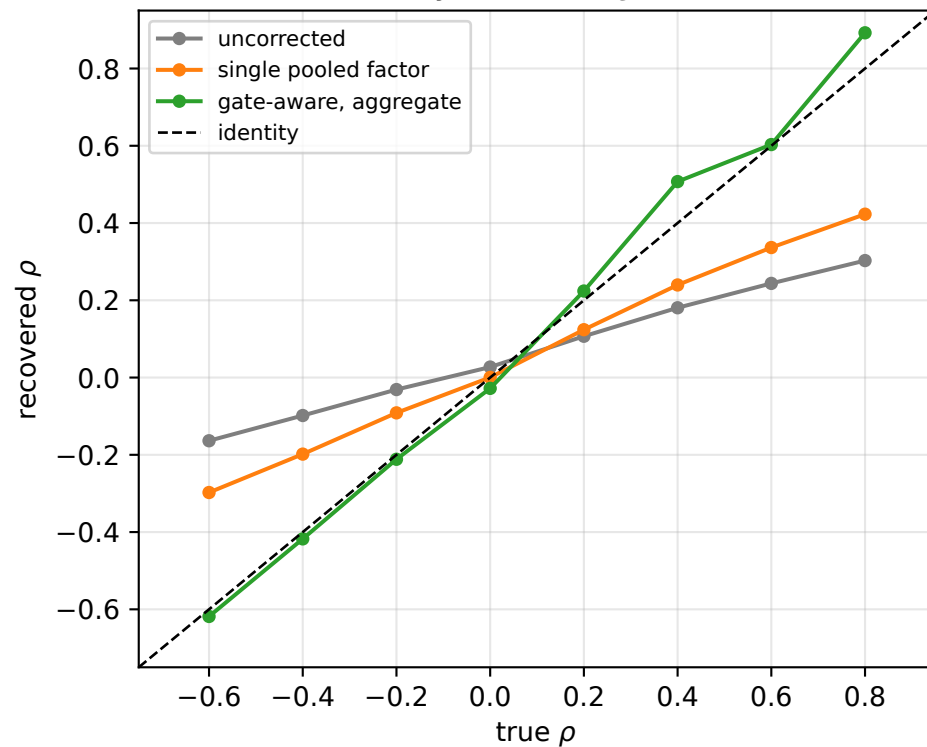
Recovery, K=300 , r_e=0.0276
