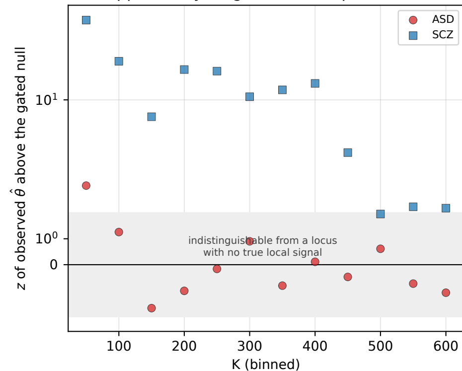
Applicability diagnostic, 78 reported loci
