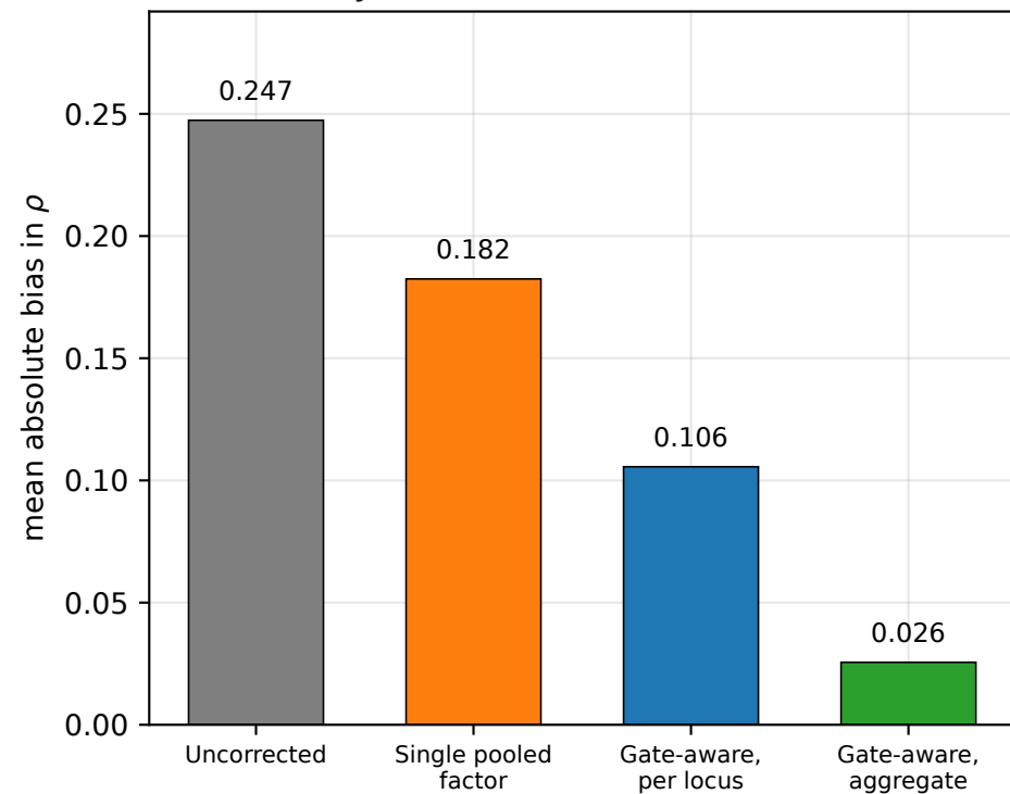
Bias by estimator (48 simulation cells)
