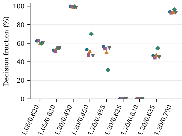
(c) Zero-regret frequency
