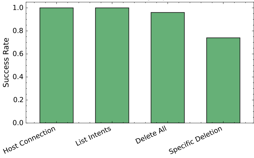
Success Rate by Operation
