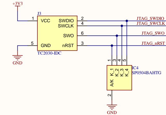
SWD_JTAG
