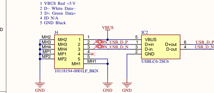
USB Connector
