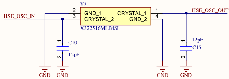
High frequency oscillator
