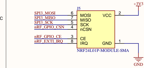
Wireless Module
