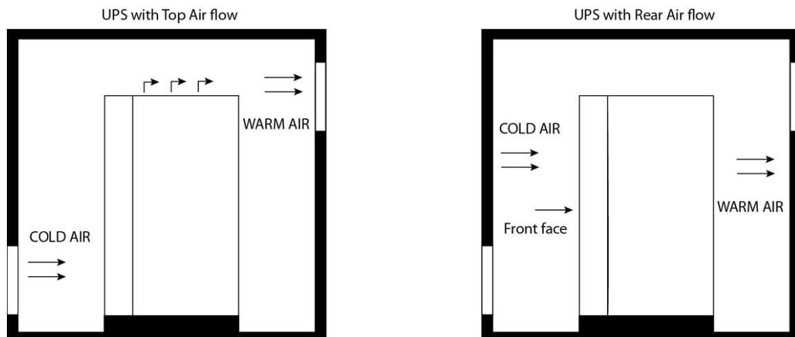
Cross Ventilation of UPS Room
