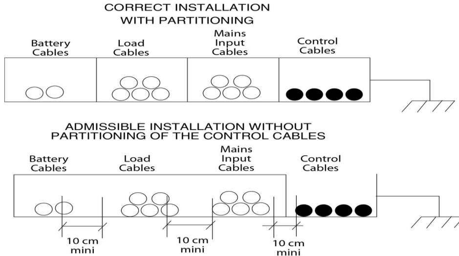
Typical Cable laying scheme
