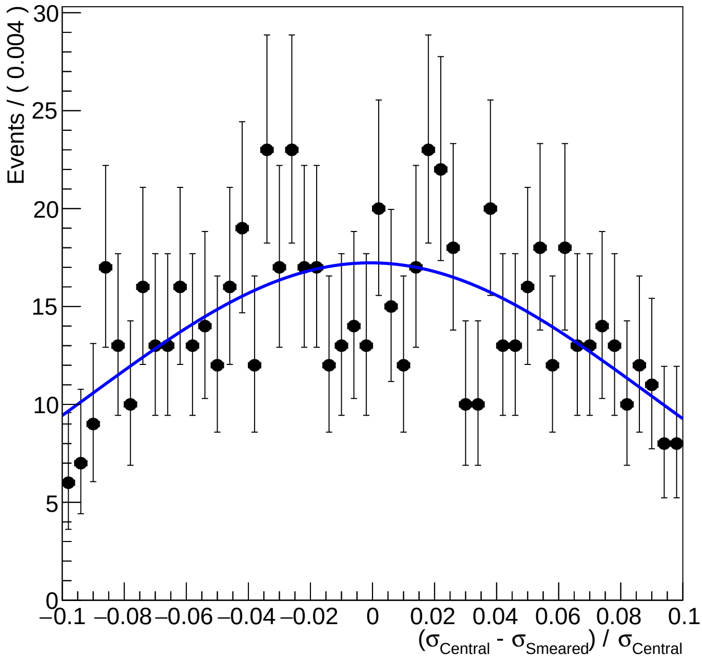
Relative difference between central and smeared value in 33th mass bin
