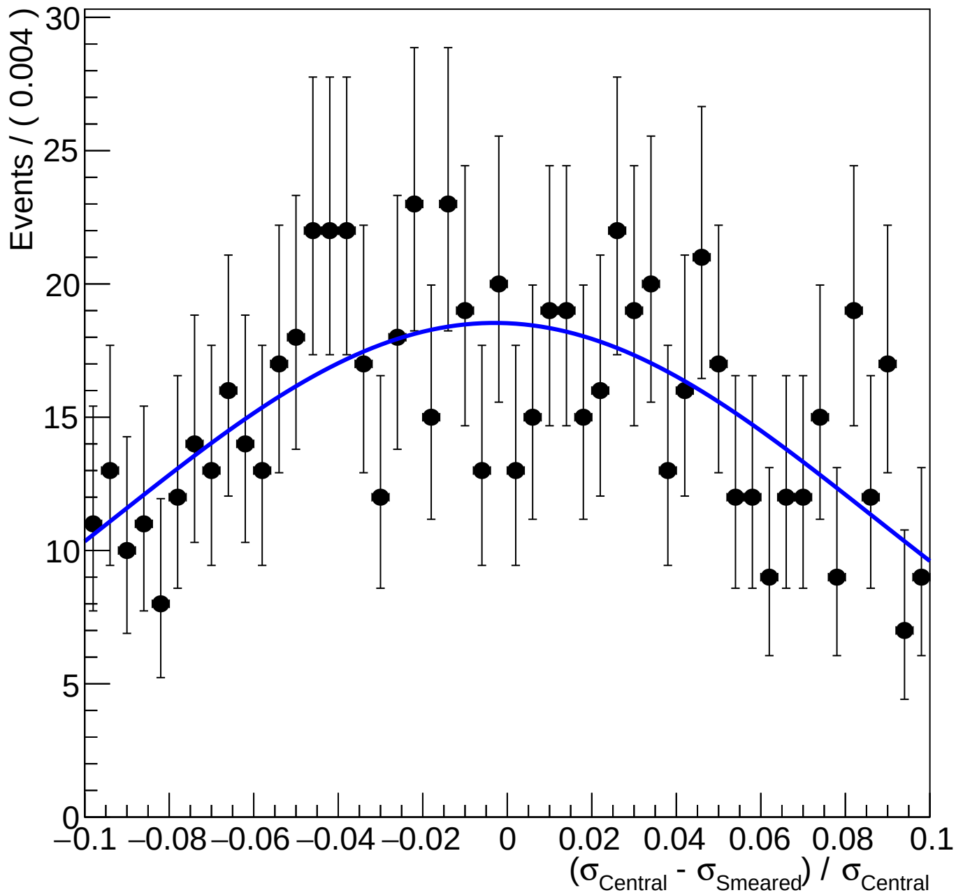
Relative difference between central and smeared value in 34th mass bin
