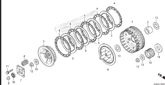
E-8 CLUTCH
