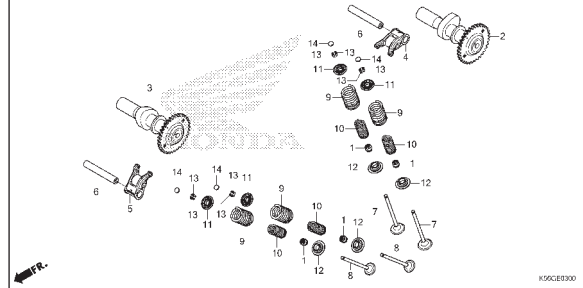
E-3 CAMSHAFT/VALVE
