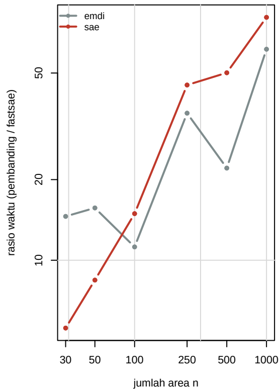
(b) Fay–Herriot spasial
