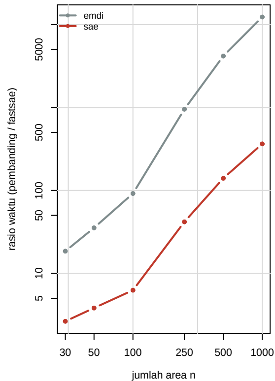
(a) Fay–Herriot area-level
