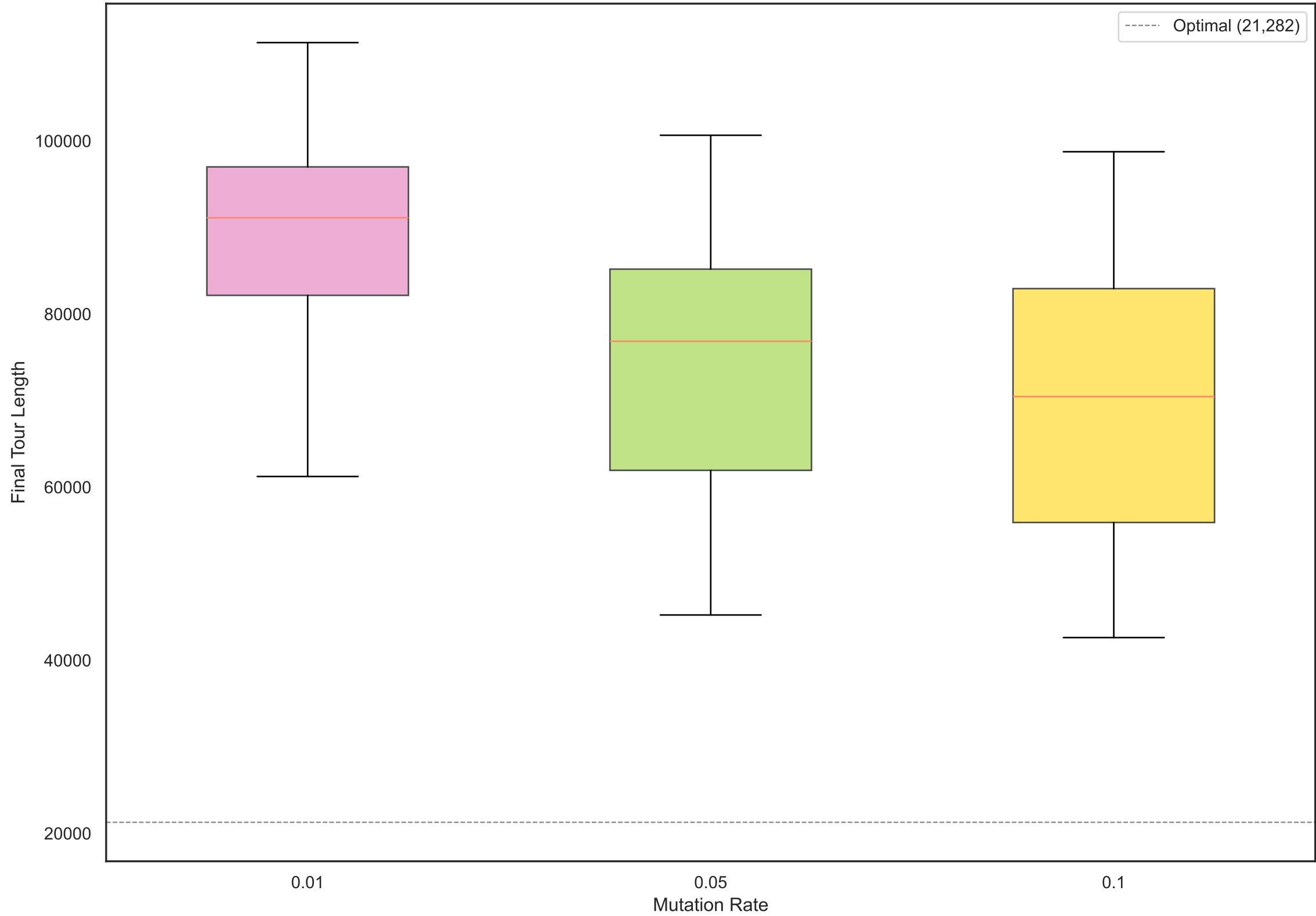
Solution Quality by Mutation Rate (naive crossover, repair enabled, 30 seeds per config)
