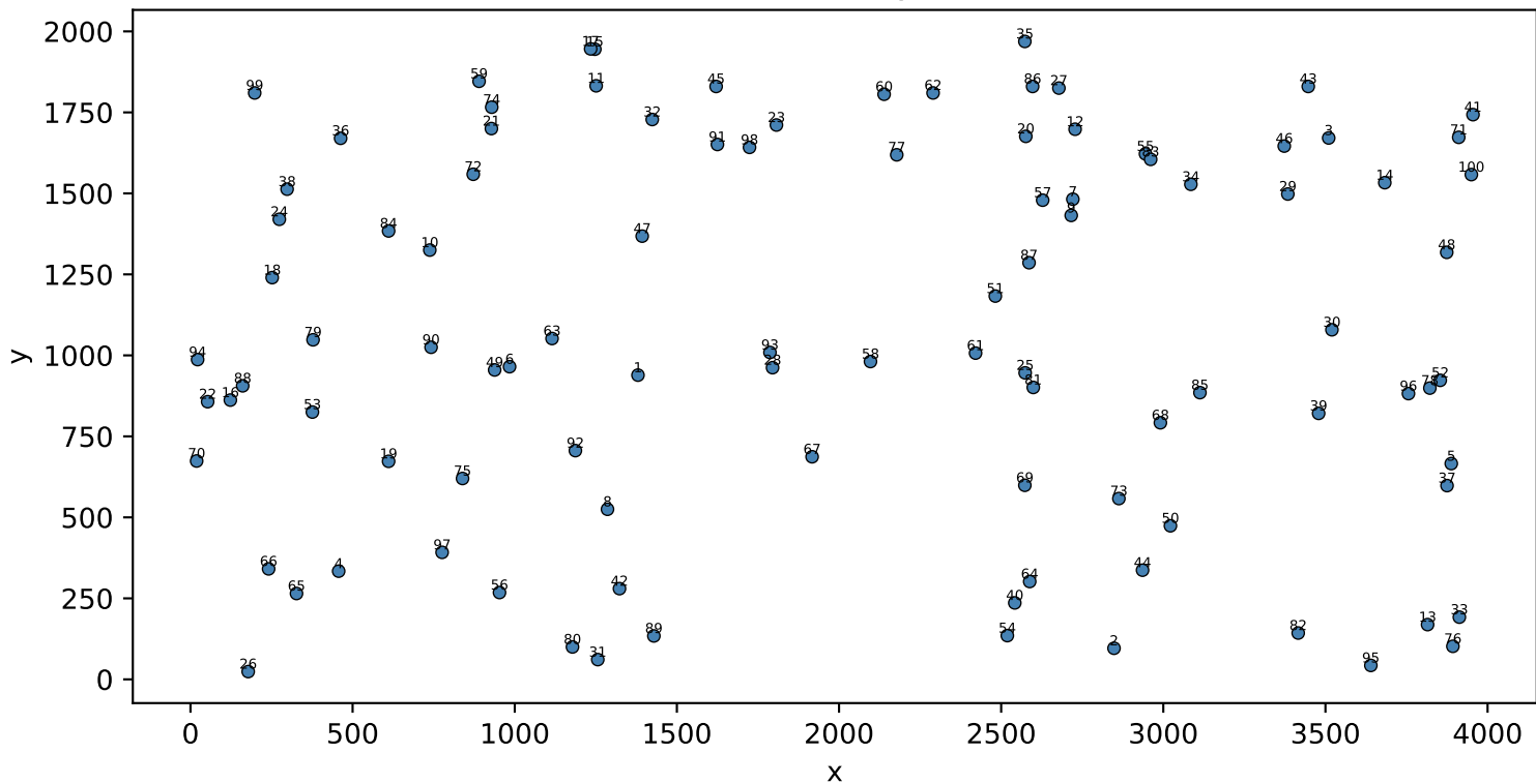
kroA100 — 100 City Locations
