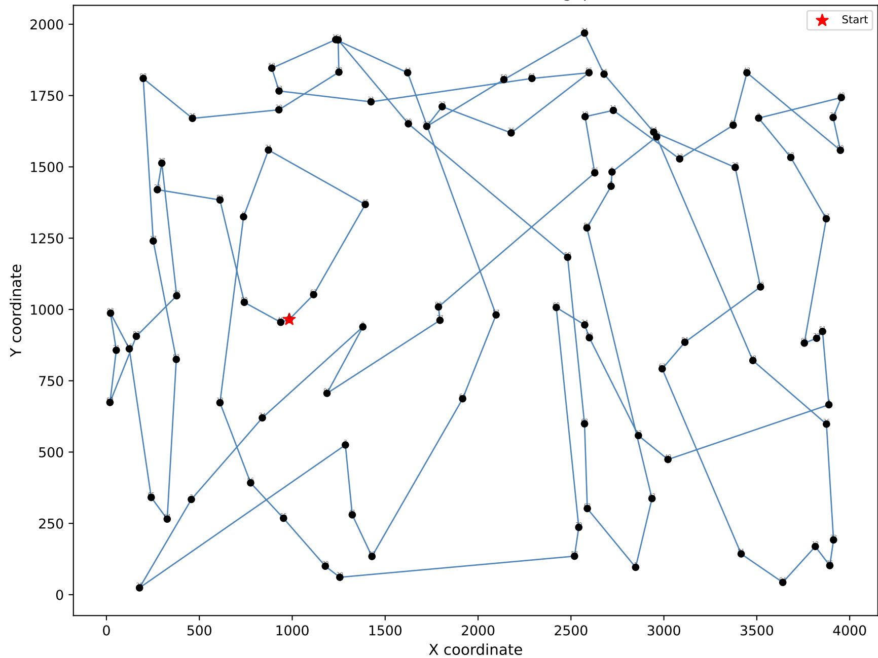
Best Tour Found (fitness=37,956, gap=78.3%)
