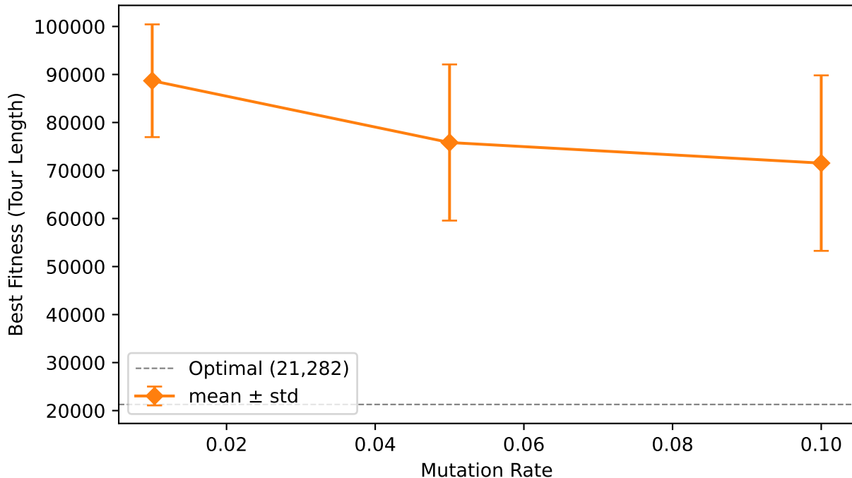
Effect of Mutation Rate on Solution Quality
