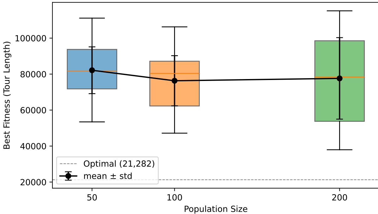
Effect of Population Size on Solution Quality
