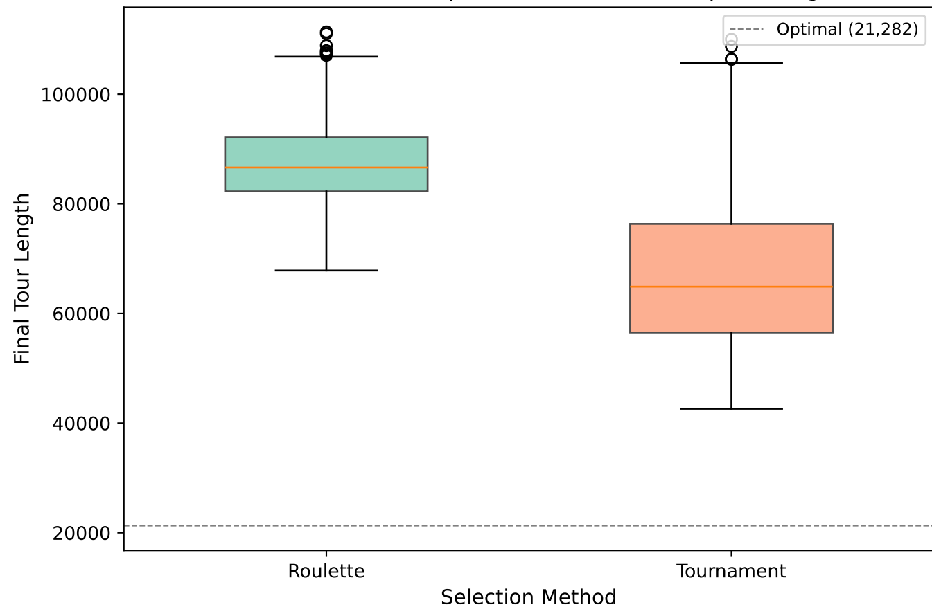
Solution Quality by Selection Method (naive crossover, repair enabled, 30 seeds per config)
