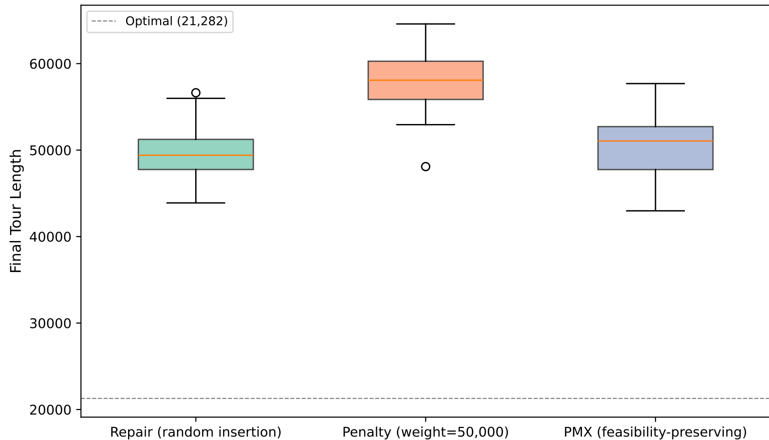
Solution Quality by Constraint-Handling Strategy (kroA100, 30 runs)
