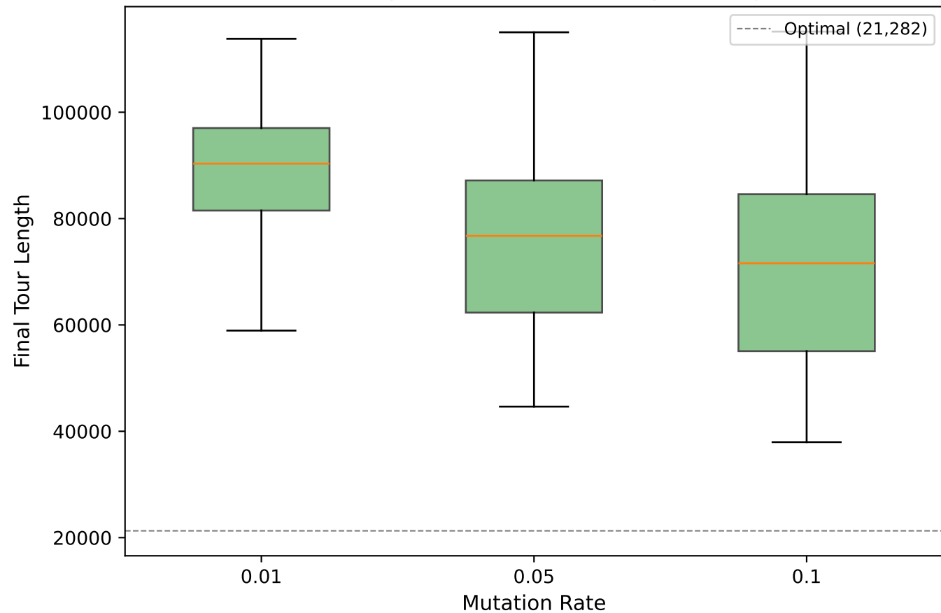
Solution Quality by Mutation Rate (PMX, repair enabled, 30 seeds per config)
