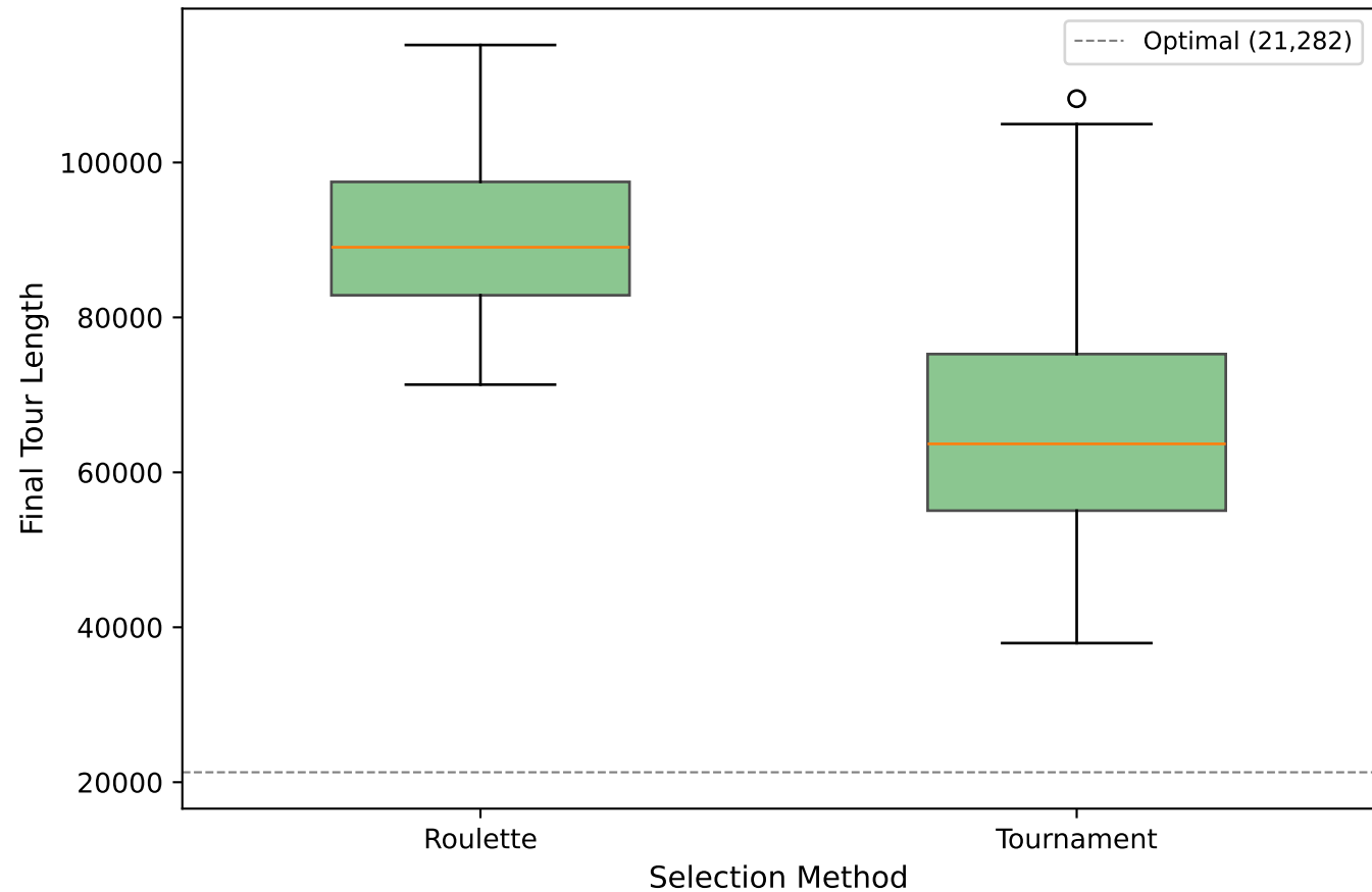
Solution Quality by Selection Method (PMX, repair enabled, 30 seeds per config)
