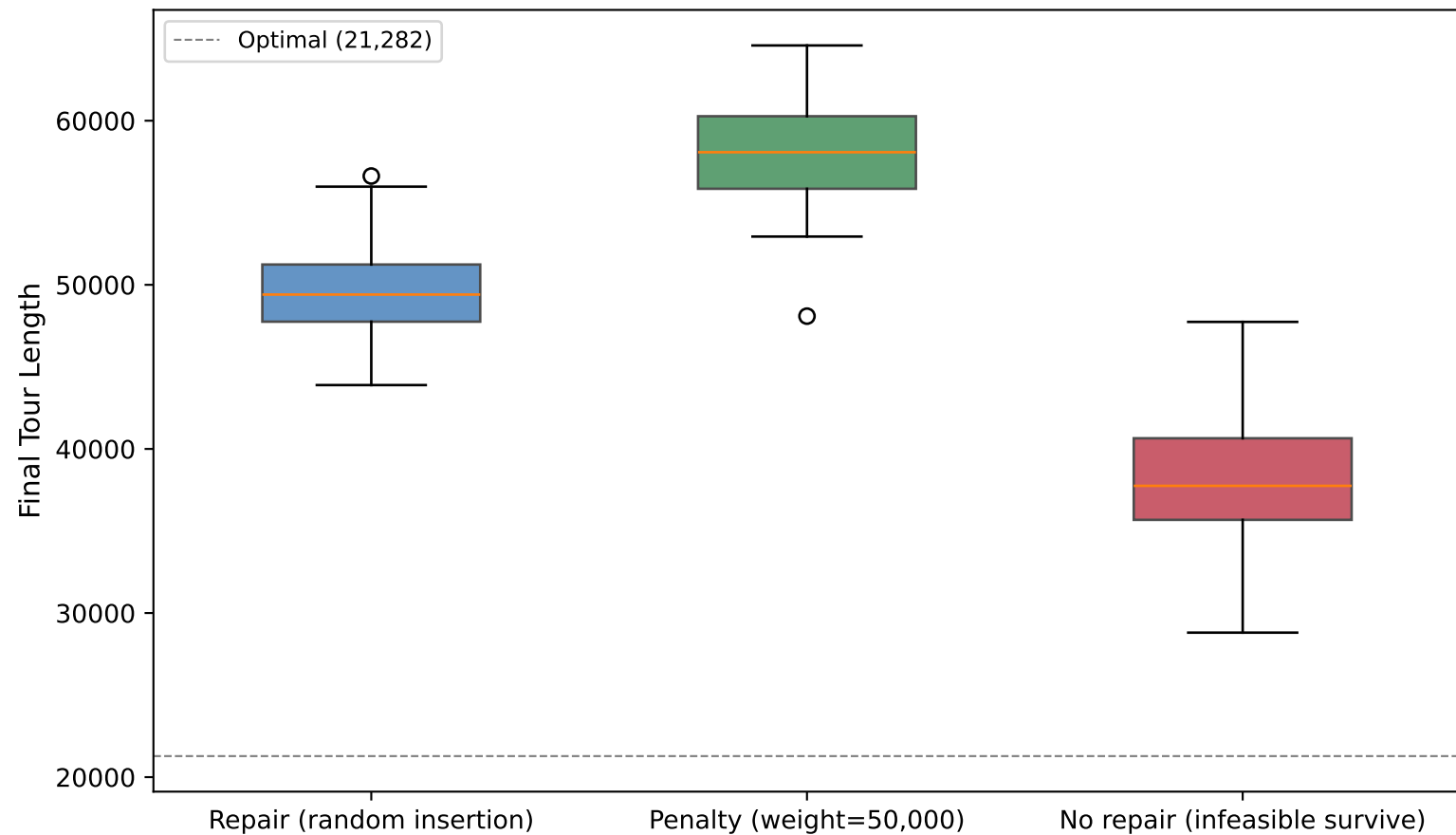
Solution Quality by Constraint-Handling Strategy (kroA100, naive crossover, 30 runs)
