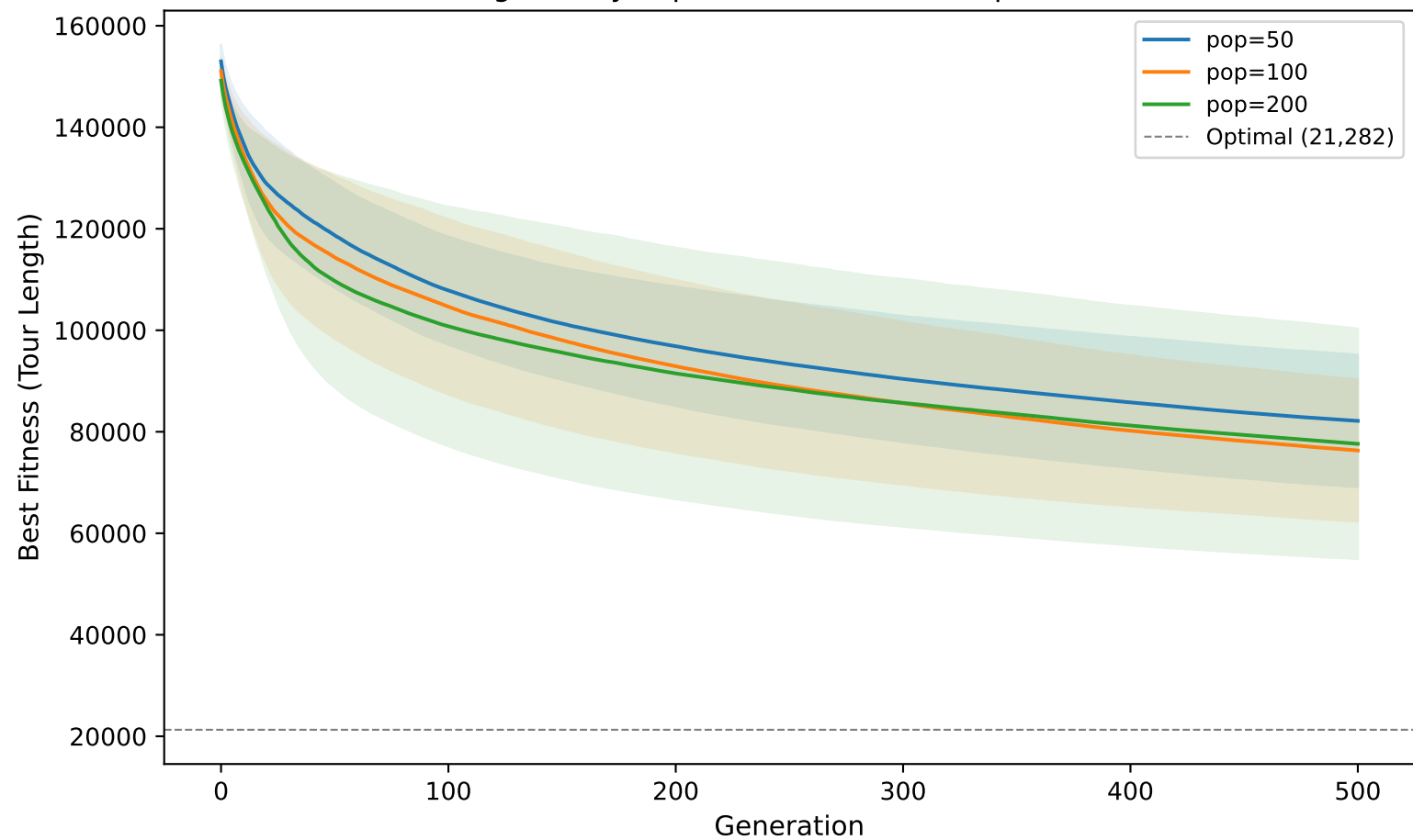
Convergence by Population Size (PMX, repair enabled)
