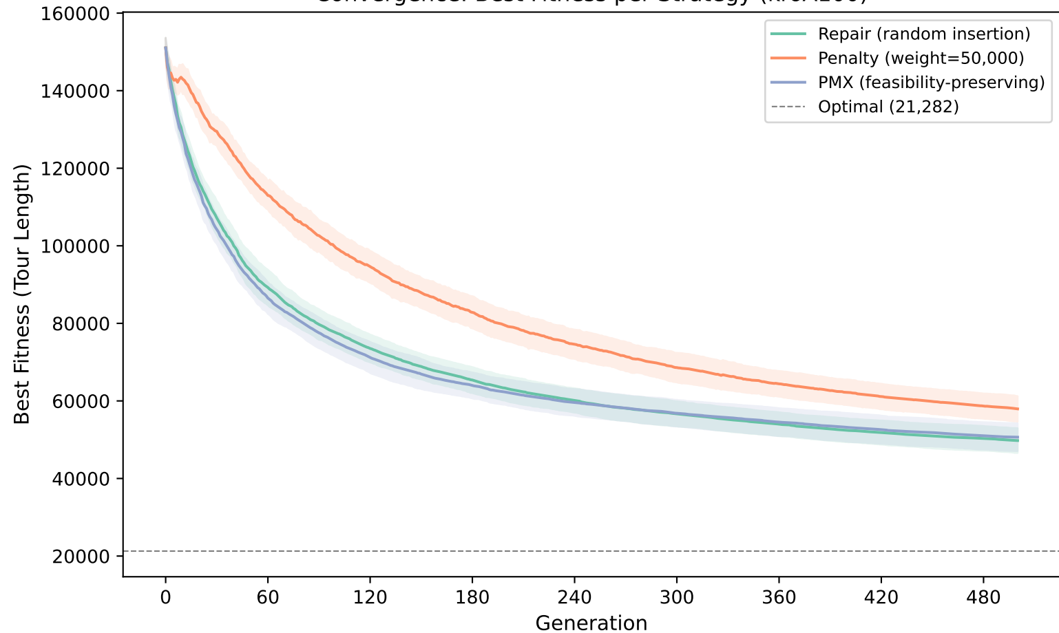
Convergence: Best Fitness per Strategy (kroA100)
