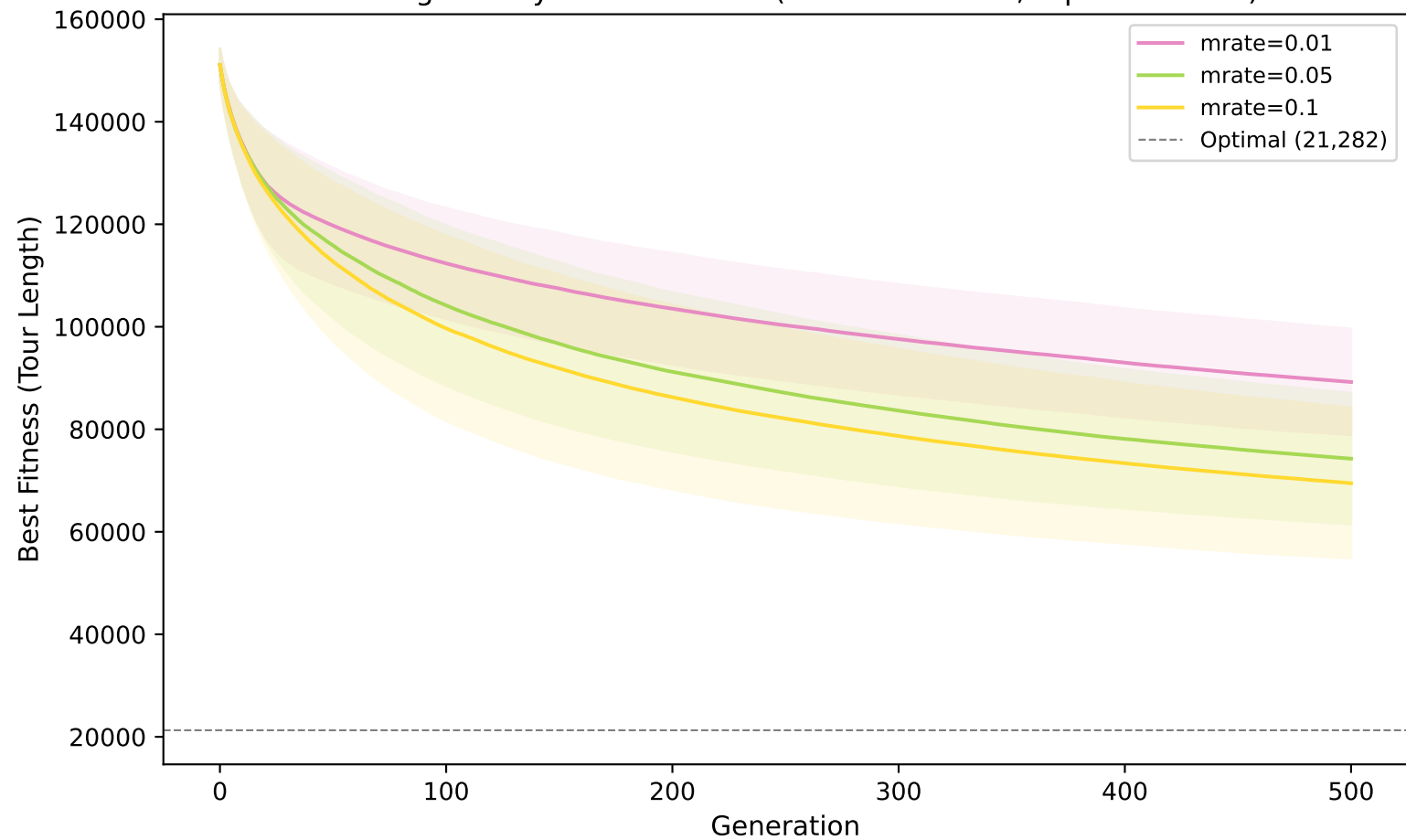
Convergence by Mutation Rate (naive crossover, repair enabled)
