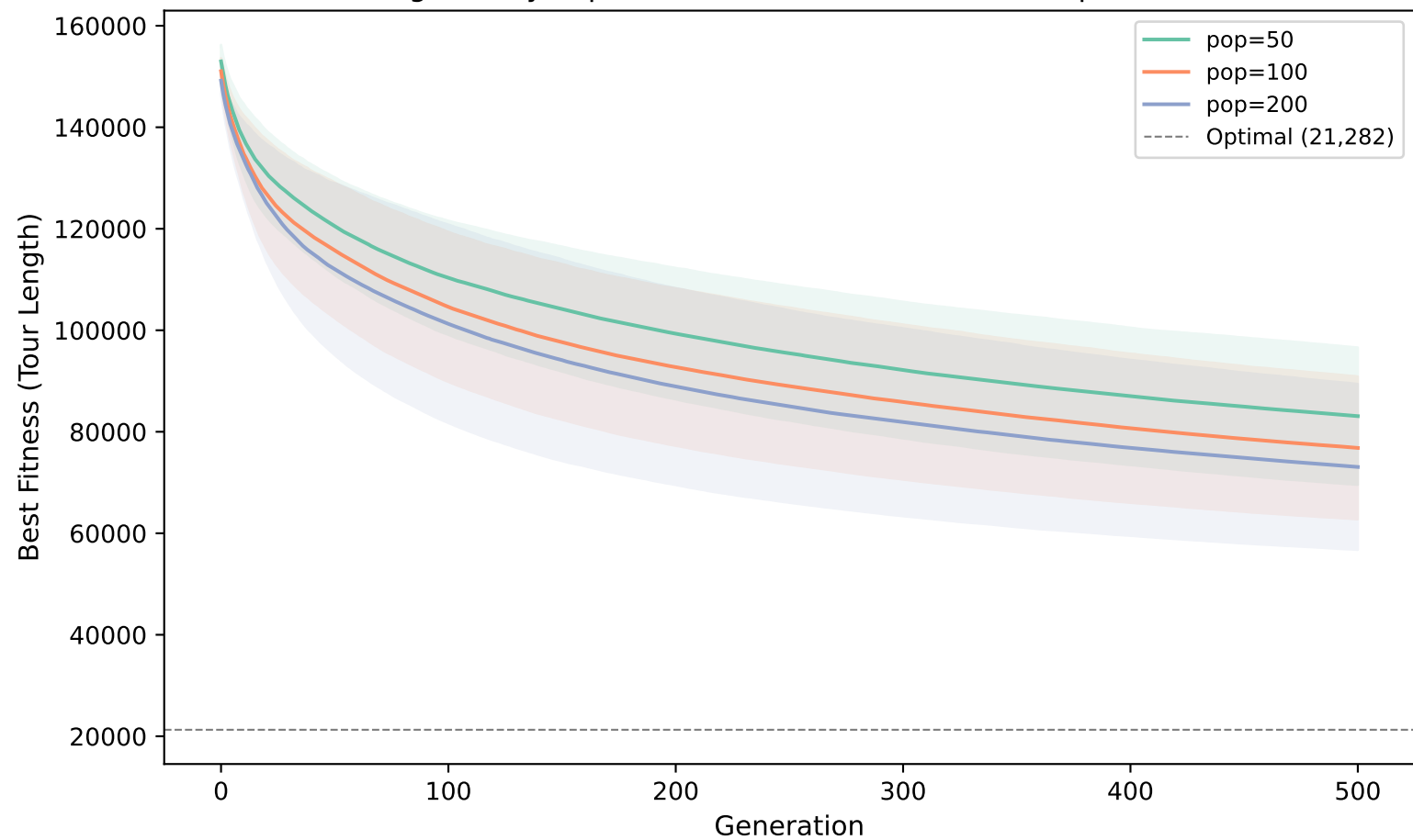
Convergence by Population Size (naive crossover, repair enabled)
