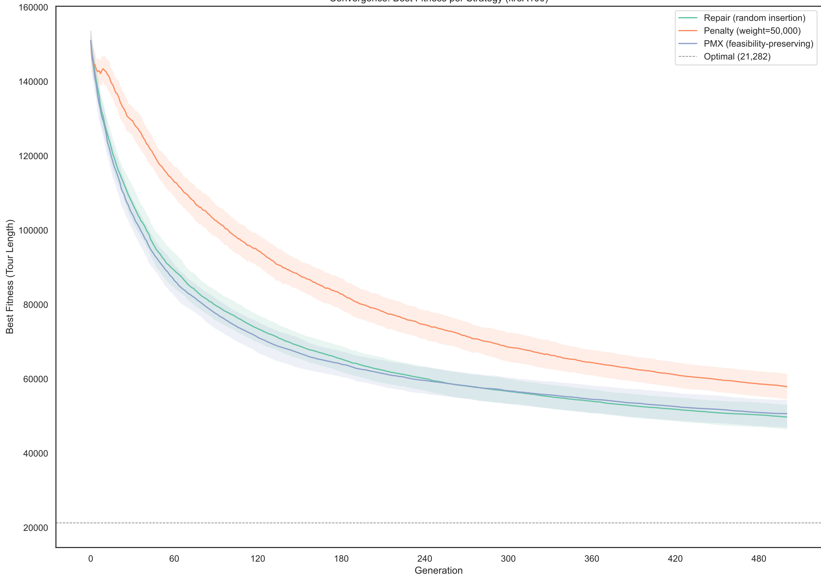
Convergence: Best Fitness per Strategy (kroA100)
