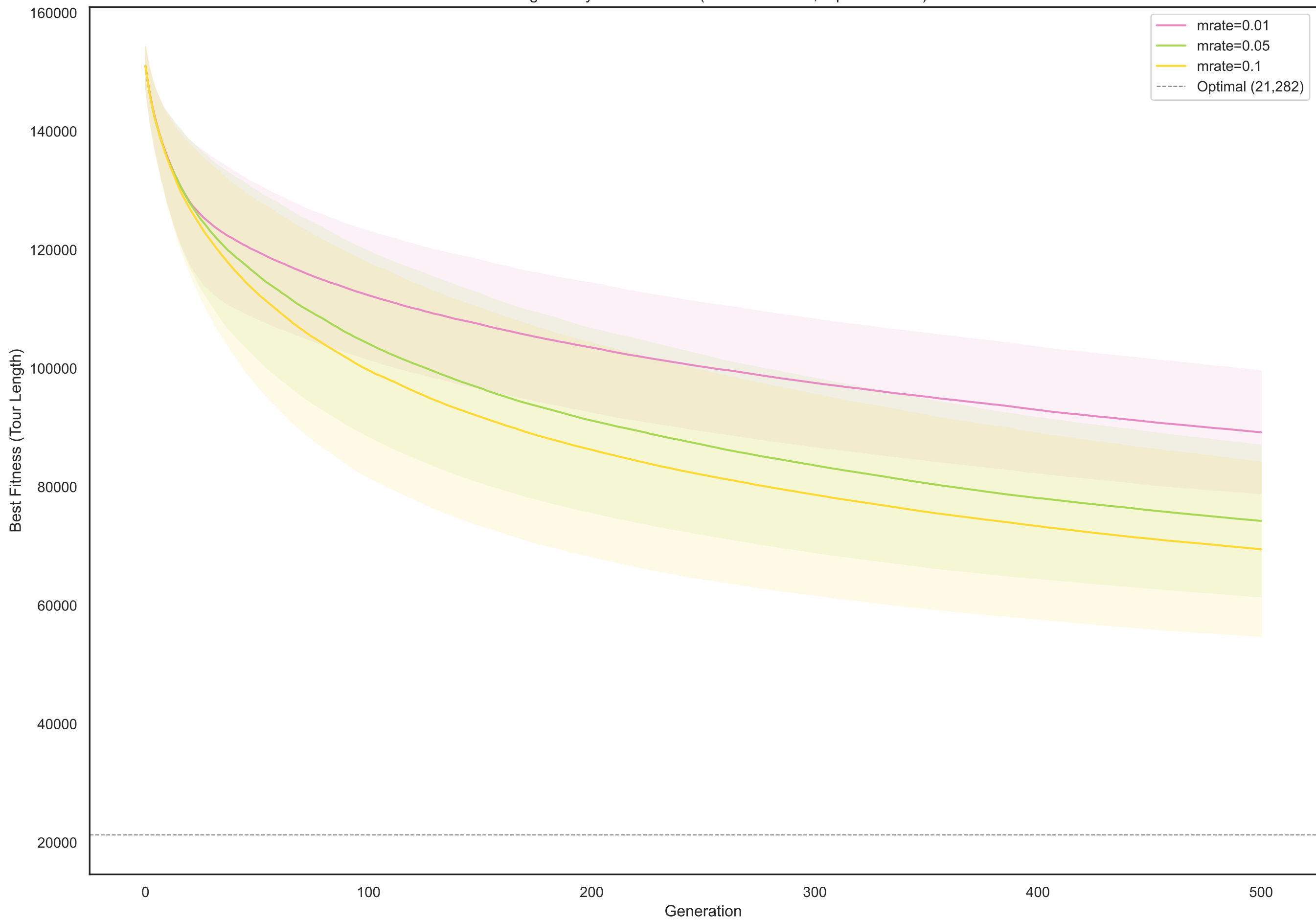
Convergence by Mutation Rate (naive crossover, repair enabled)
