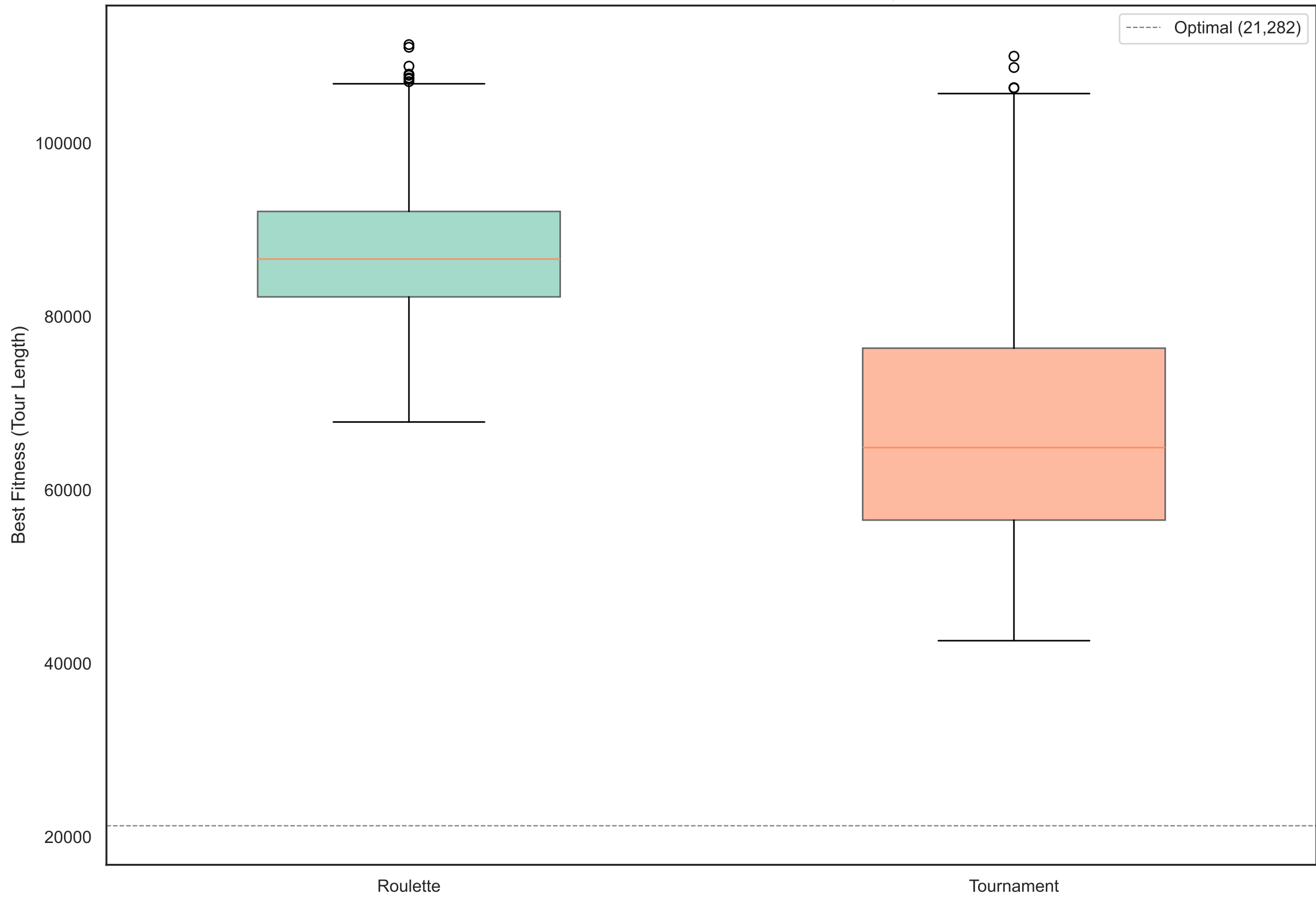
Effect of Selection Method on Solution Quality
