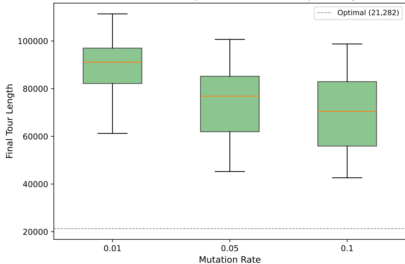
Solution Quality by Mutation Rate (naive crossover, repair enabled, 30 seeds per config)
