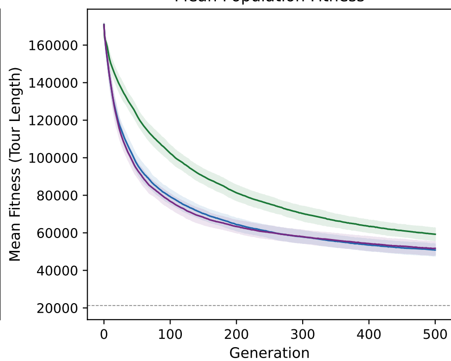
Mean Population Fitness
