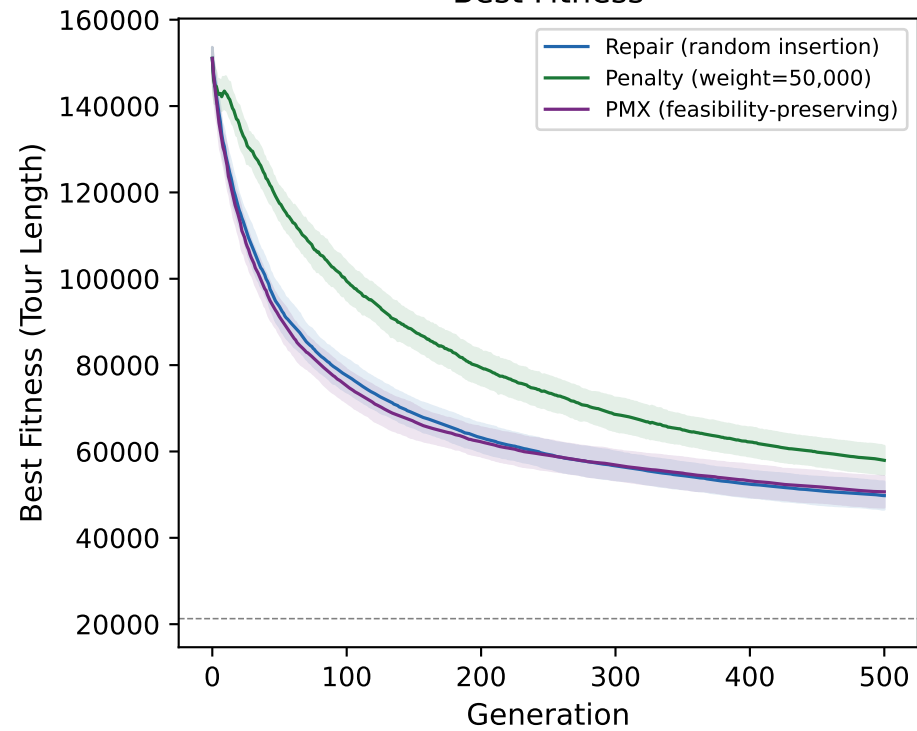
Best Fitness
