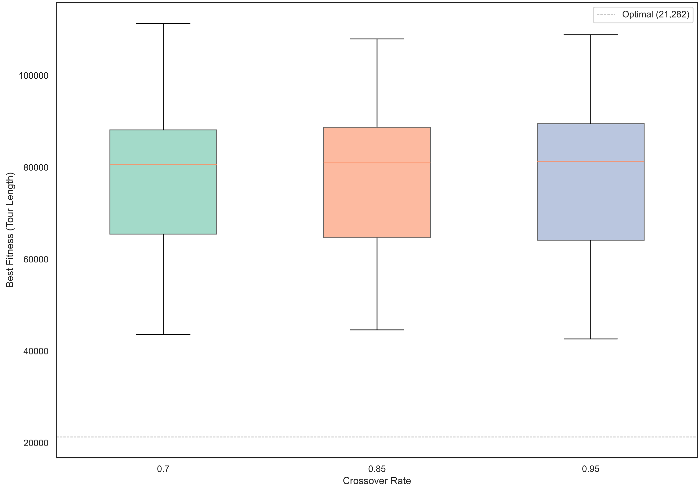
Effect of Crossover Rate on Solution Quality
