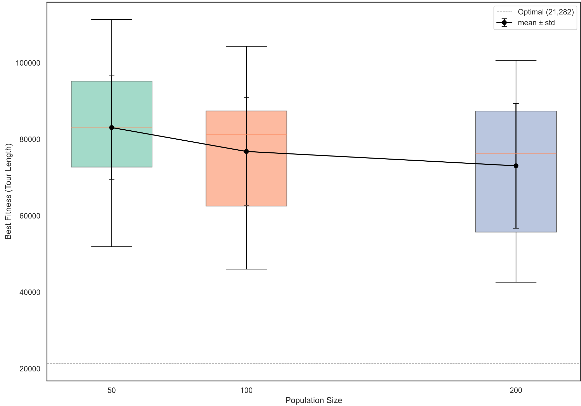
Effect of Population Size on Solution Quality
