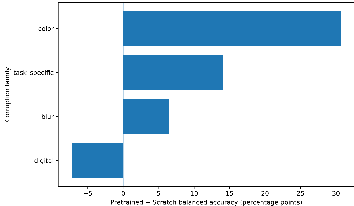
BloodMNIST: effect of ImageNet pretraining
