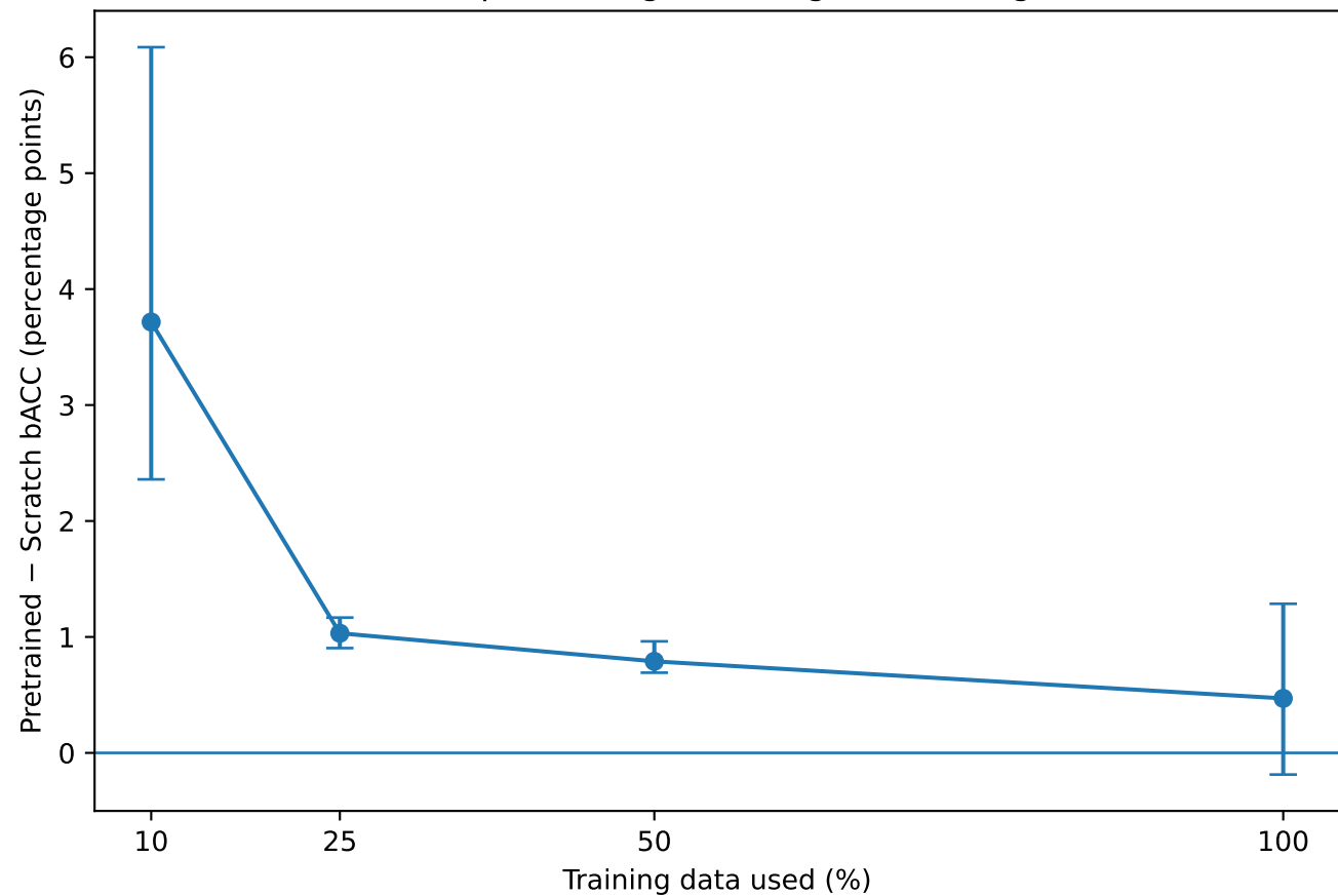
BloodMNIST: pretraining advantage vs training-set size
