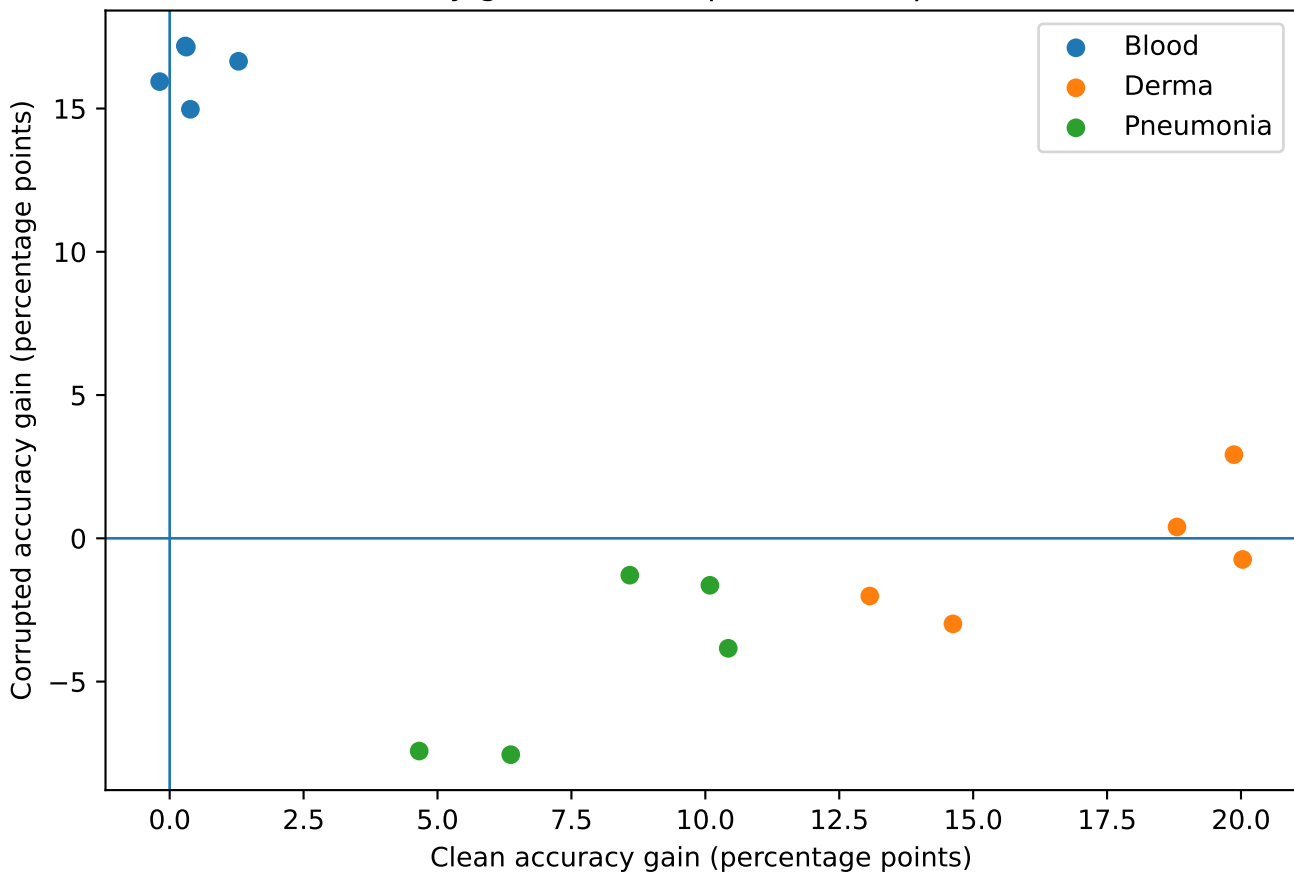
Clean accuracy gain does not predict corruption robustness
