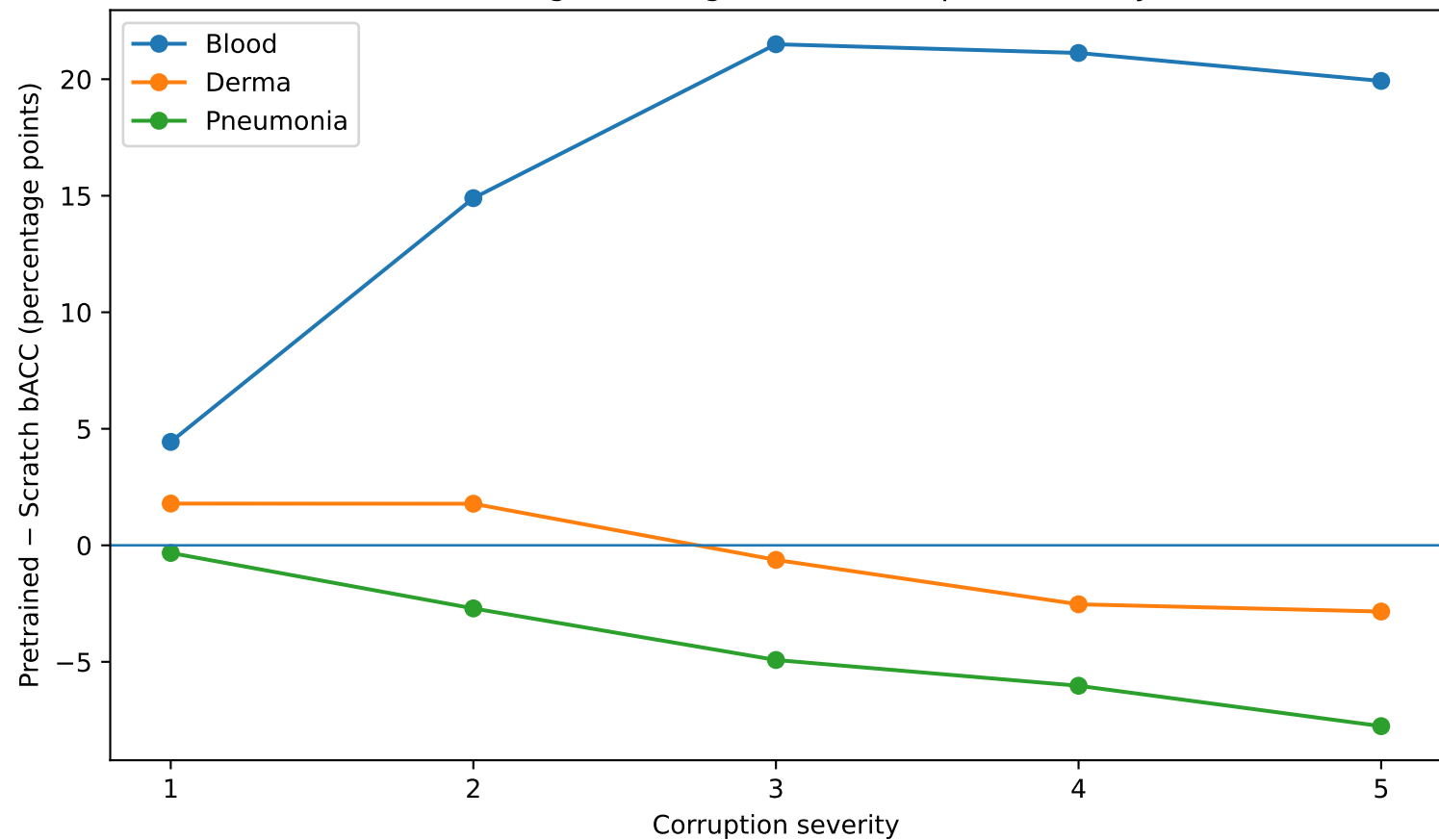
Pretraining advantage across corruption severity
