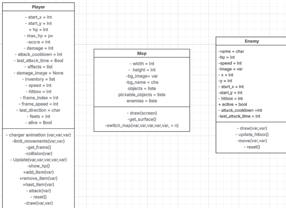
Figure 8: Diagramme de classes 1
