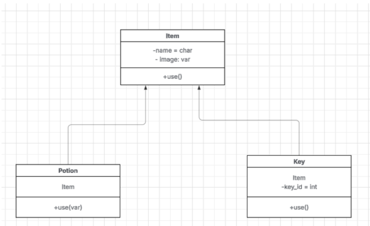
Figure 11: Diagramme de classes 4
