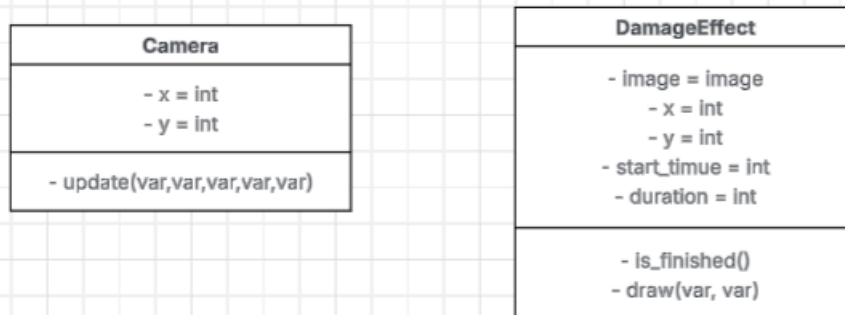
Figure 8: Diagramme de classes 1
