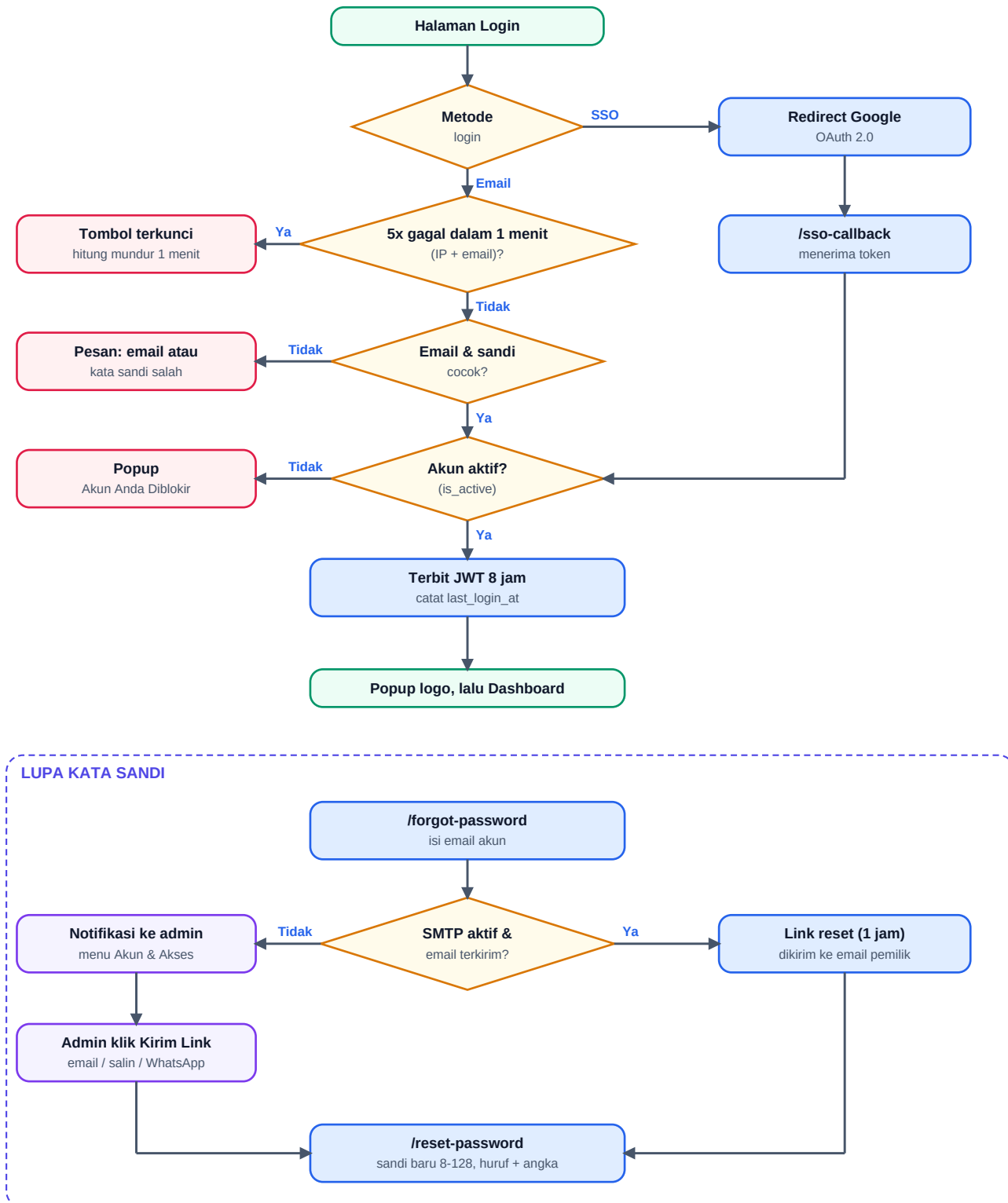
Gambar 7. Flowchart login email/sandi, login SSO Google, dan lupa kata sandi
