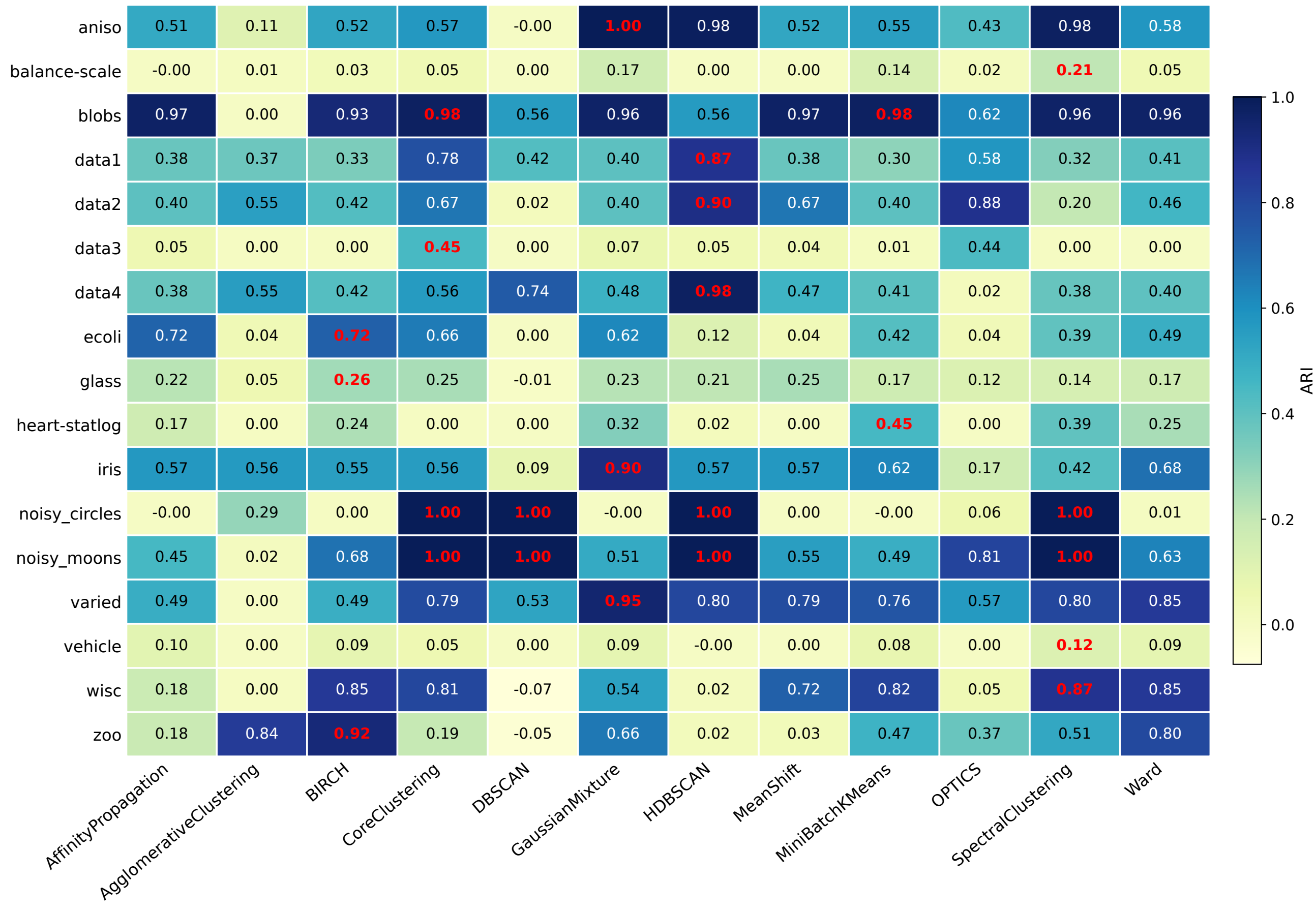
Adjusted Rand Index (ARI) across algorithms and datasets
