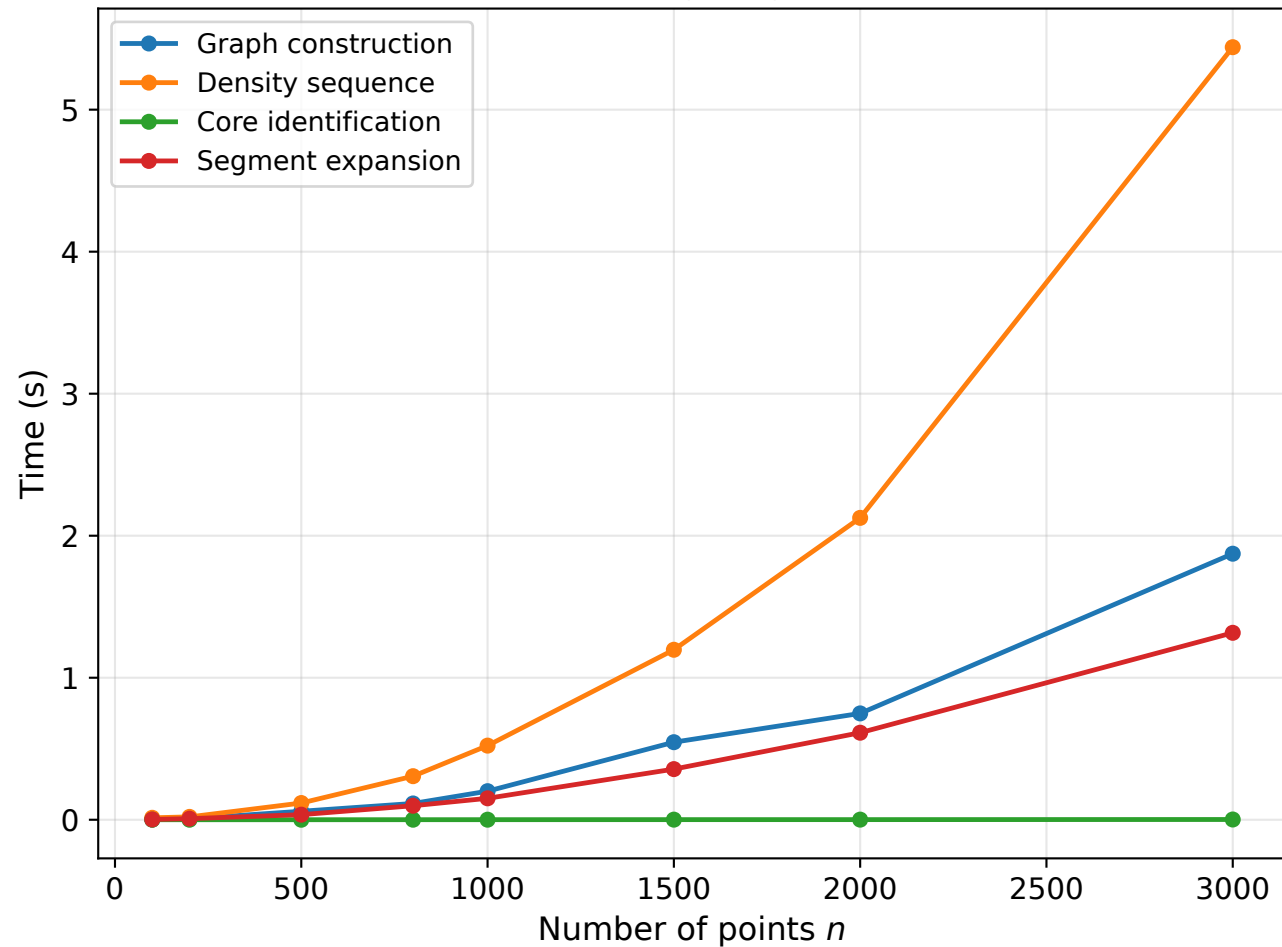
(a) Core Clustering stage breakdown
