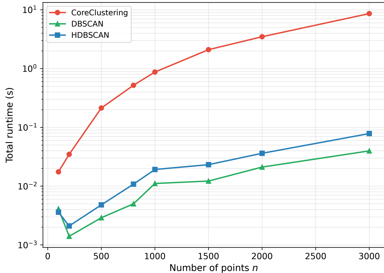
(b) Total runtime vs. baselines
