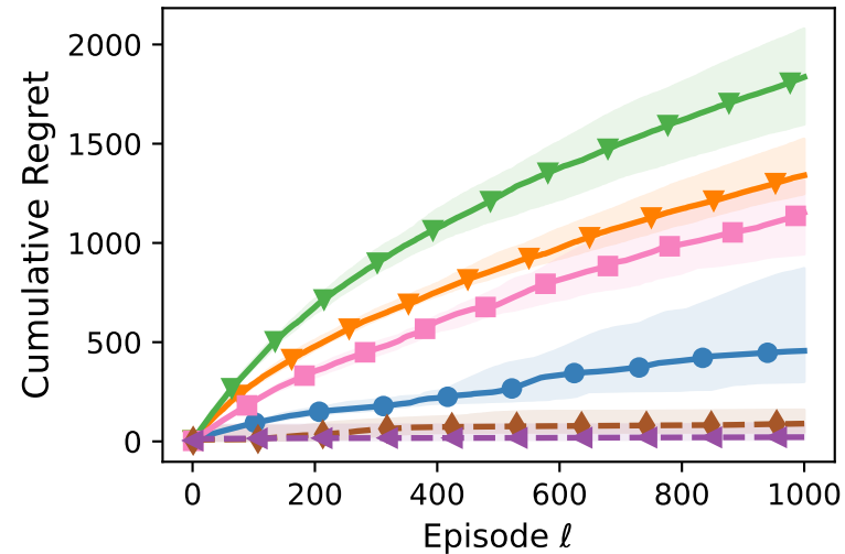
Cumulative Regret
